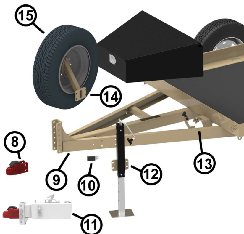
FIGURE 2-2 DRAWBAR EQUIPMENT
